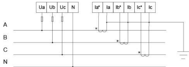
ADL300-EY Three phase four lines connect via CT
