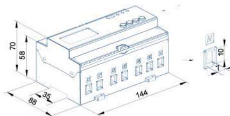
direct connect
