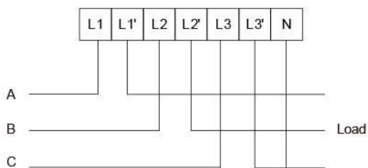
ADL300-EY Three phase four lines direct connect
